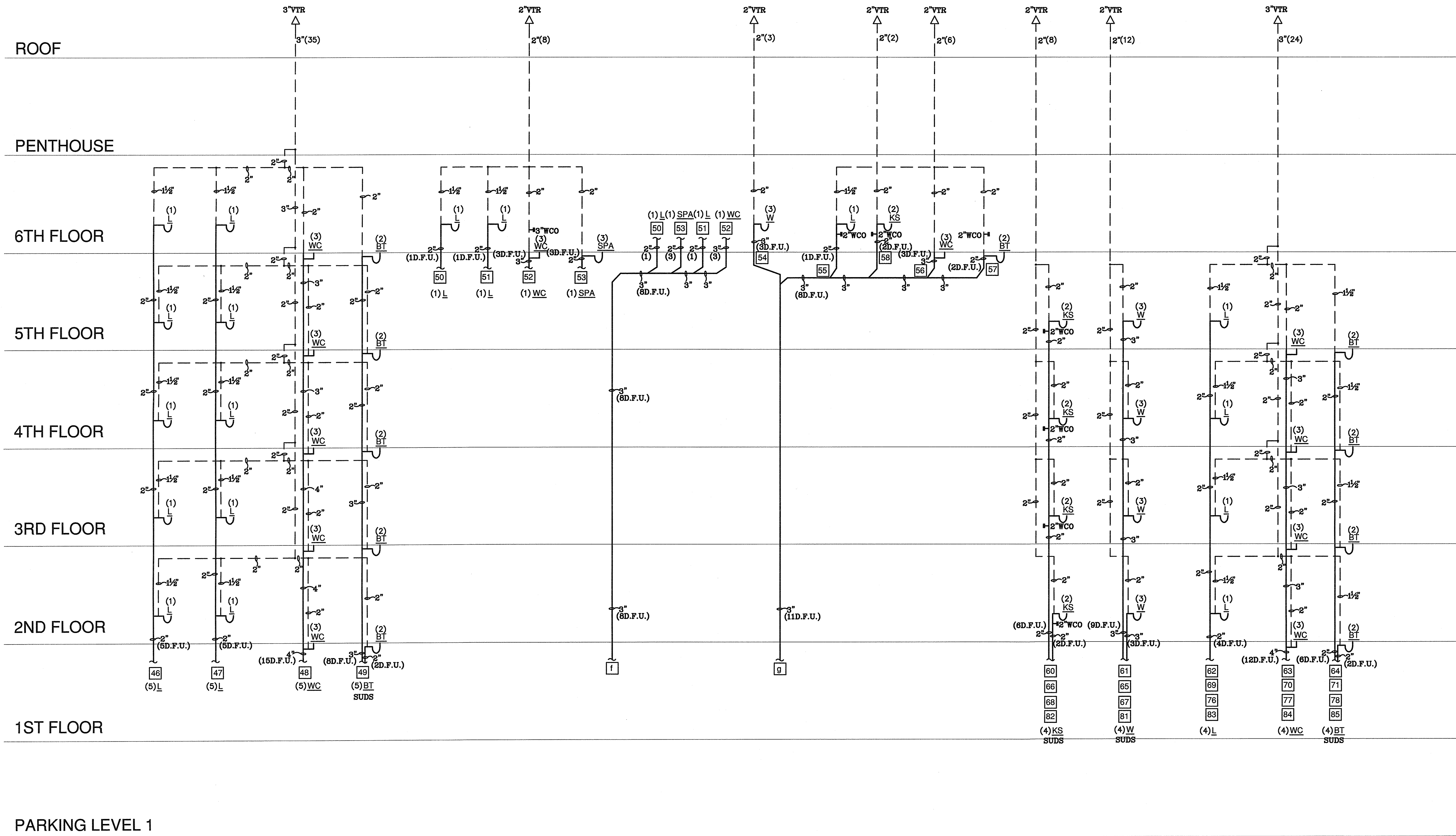
TYPICAL WASTE & VENT RISER DIAGRAM N.T.S.
